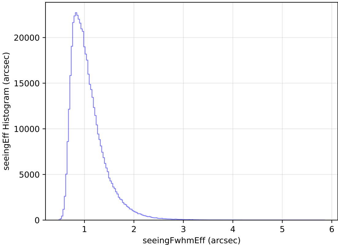
ddf_loaded_fl15_v3.4_10yrs WFD i band: seeingEff Histogram
