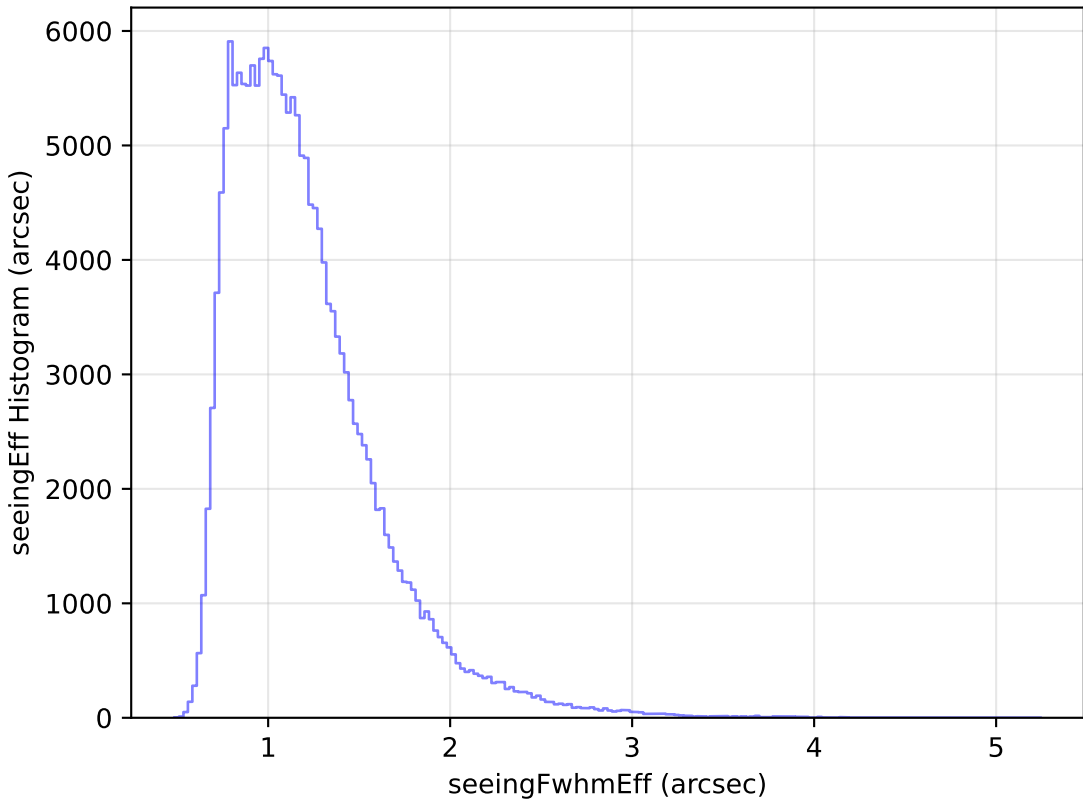
ddf_loaded_fl15_v3.4_10yrs WFD g band: seeingEff Histogram
