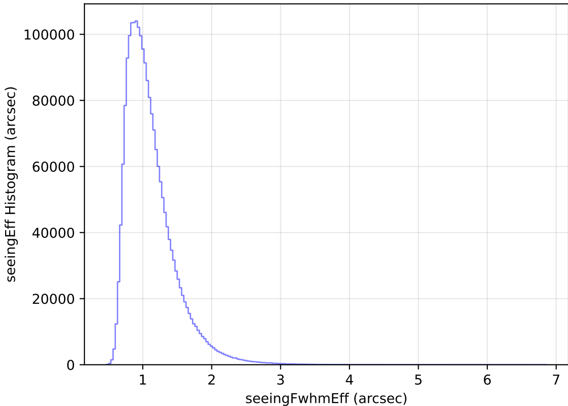
ddf_loaded_fl15_v3.4_10yrs WFD all bands: seeingEff Histogram
