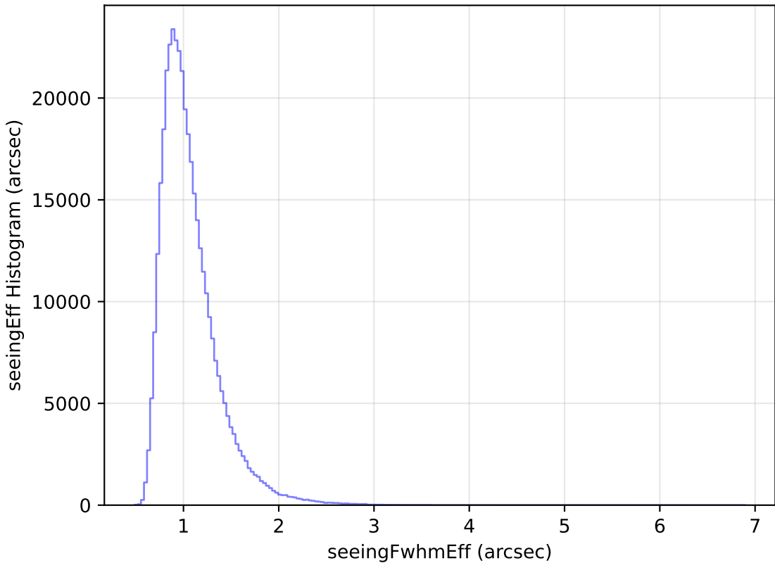
ddf_loaded_fl15_v3.4_10yrs All sky y band: seeingEff Histogram
