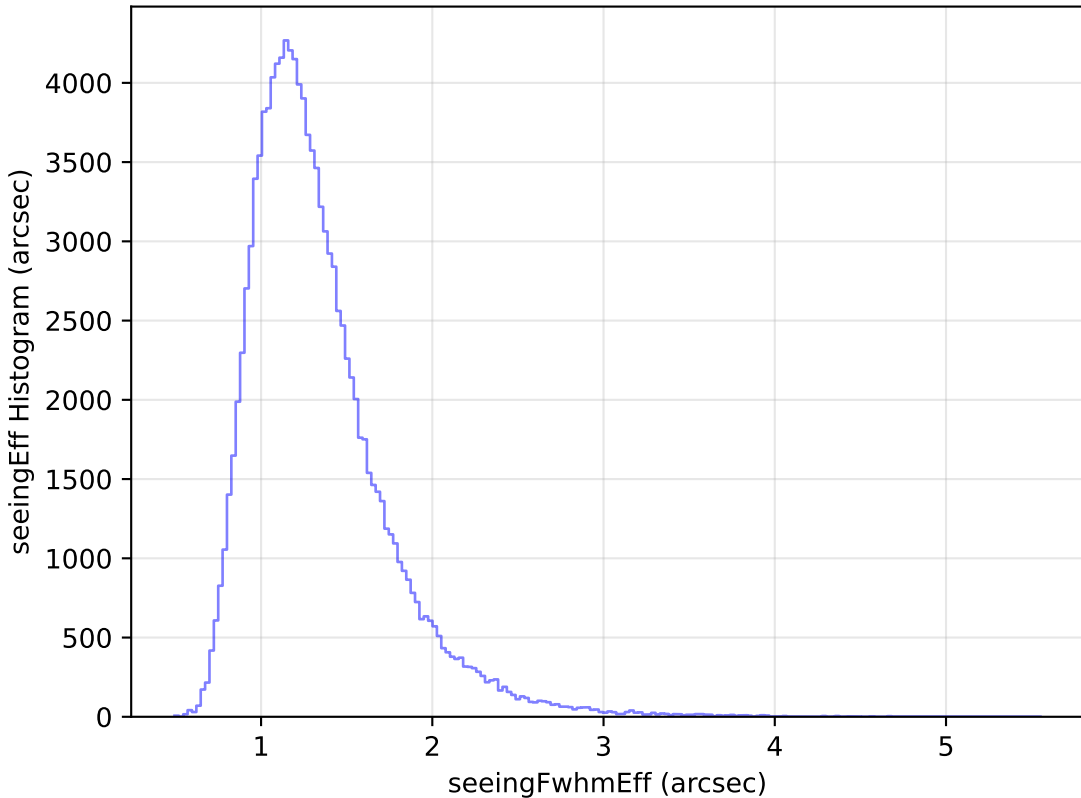
ddf_loaded_fl15_v3.4_10yrs All sky u band: seeingEff Histogram
