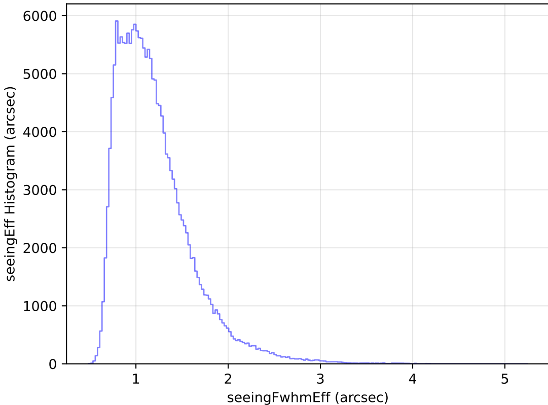
ddf_loaded_fl15_v3.4_10yrs All sky g band: seeingEff Histogram
