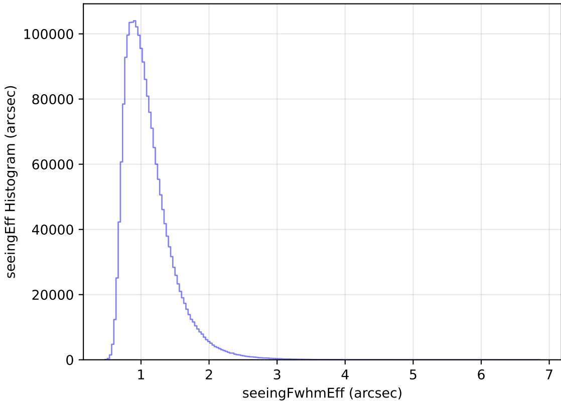
ddf_loaded_fl15_v3.4_10yrs All sky all bands: seeingEff Histogram
