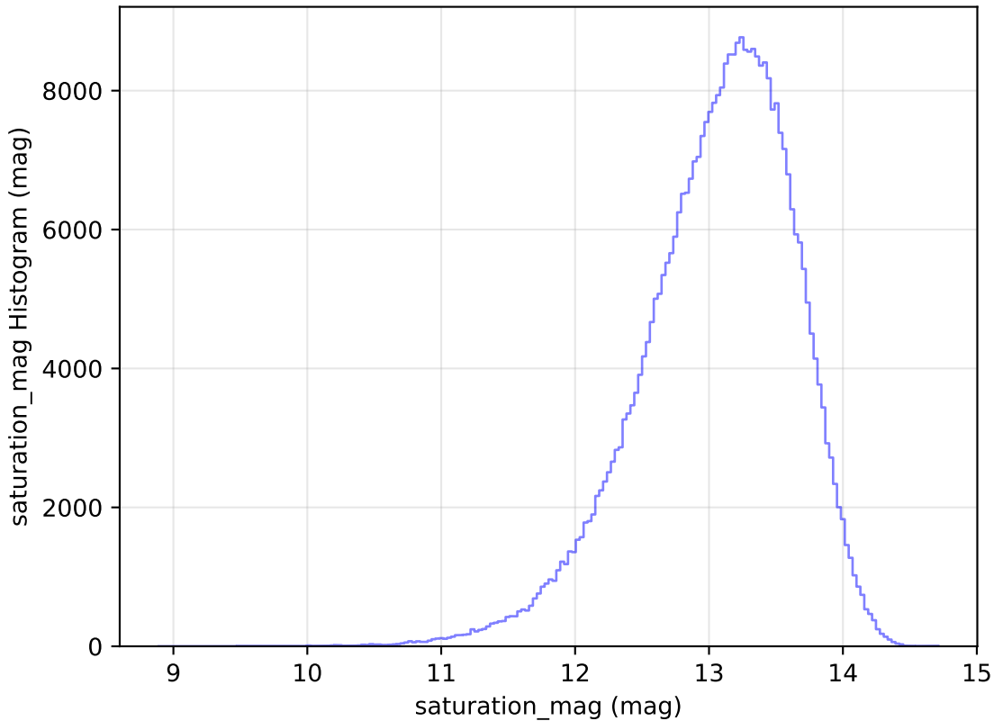
ddf_loaded_fl15_v3.4_10yrs WFD y band: saturation_mag Histogram
