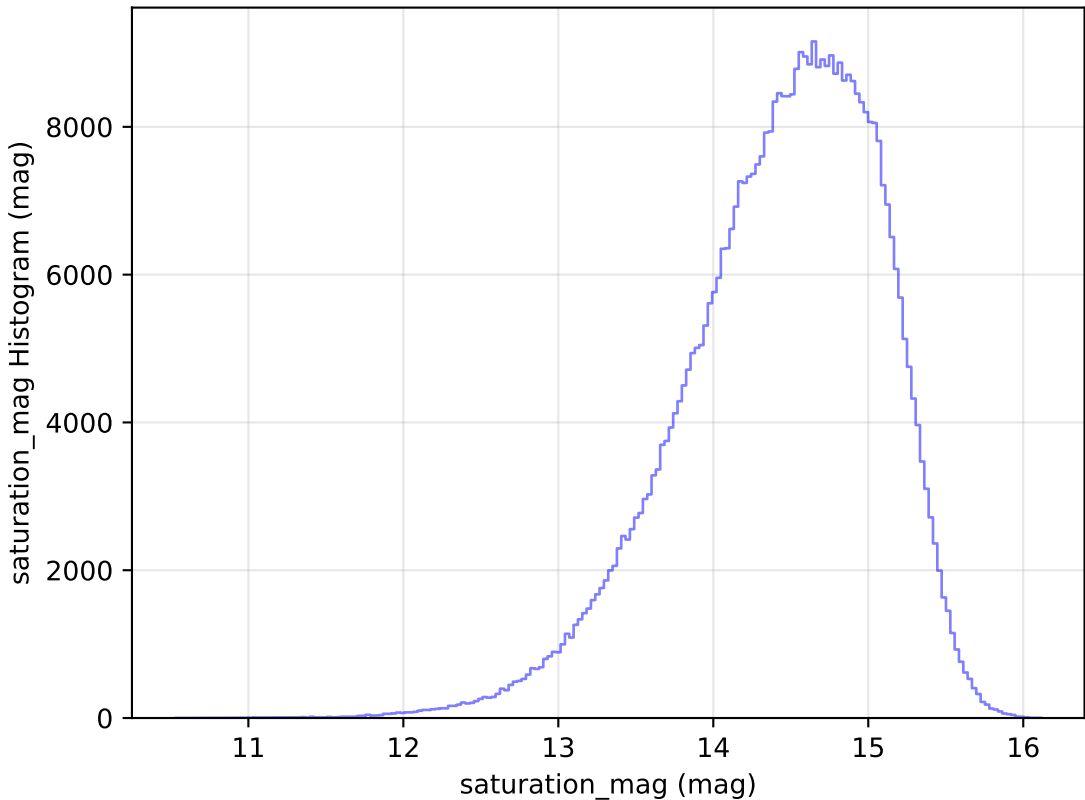
ddf_loaded_fl15_v3.4_10yrs WFD i band: saturation_mag Histogram
