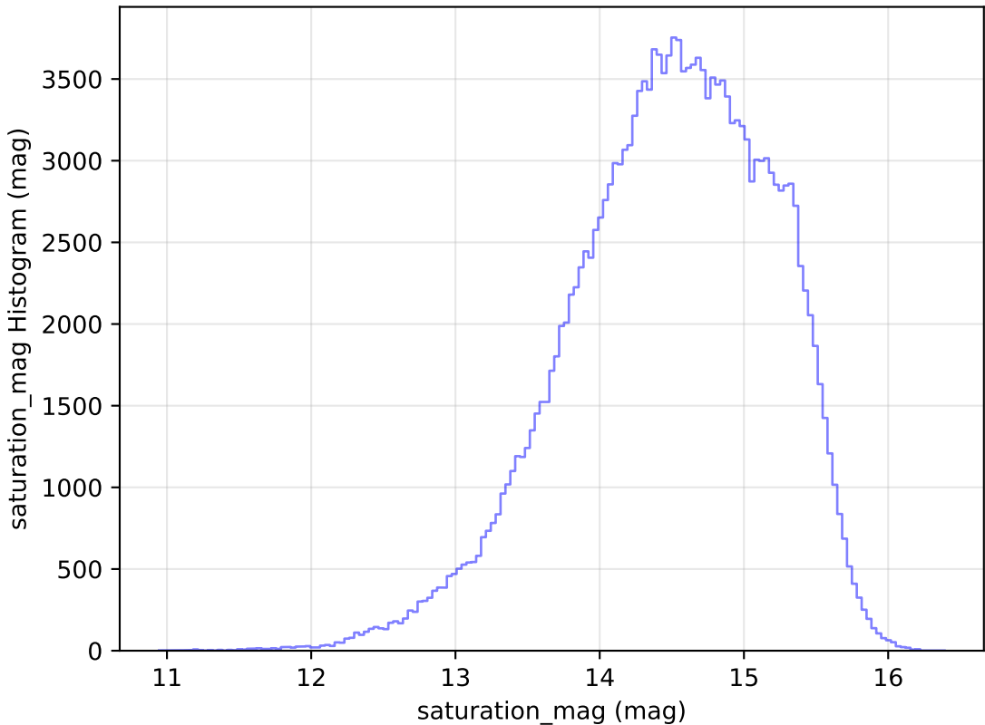
ddf_loaded_fl15_v3.4_10yrs WFD g band: saturation_mag Histogram
