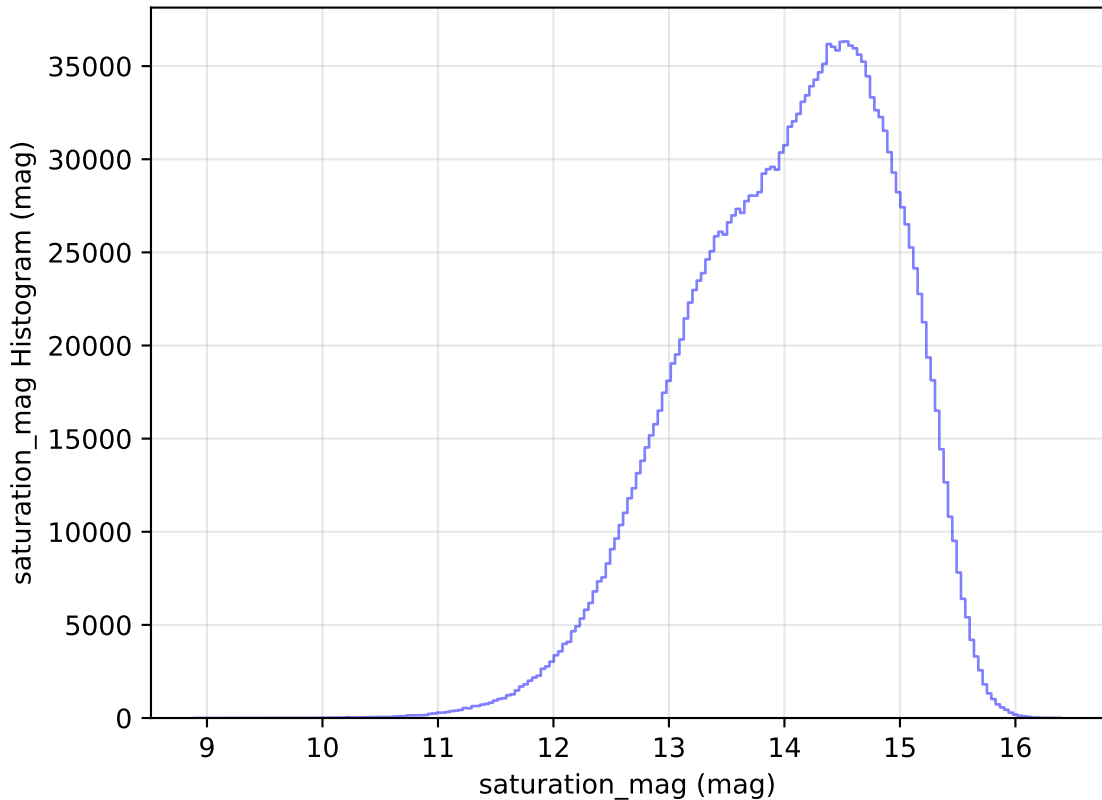
ddf_loaded_fl15_v3.4_10yrs WFD all bands: saturation_mag Histogram
