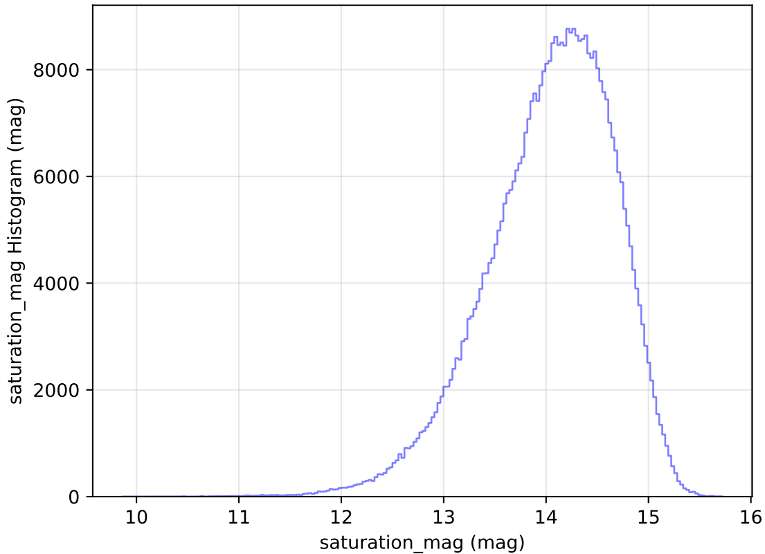
ddf_loaded_fl15_v3.4_10yrs All sky z band: saturation_mag Histogram
