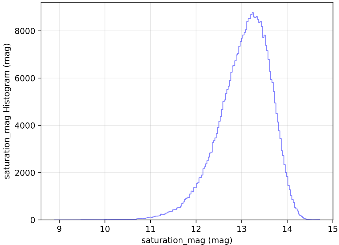
ddf_loaded_fl15_v3.4_10yrs All sky y band: saturation_mag Histogram
