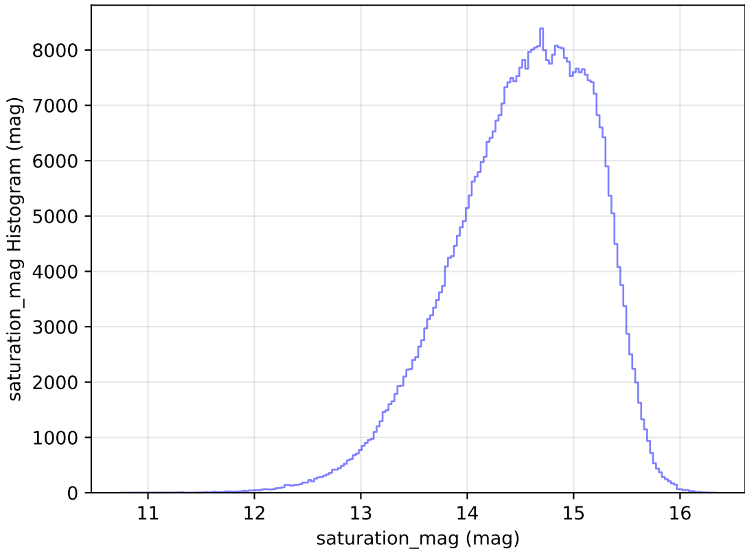
ddf_loaded_fl15_v3.4_10yrs All sky r band: saturation_mag Histogram
