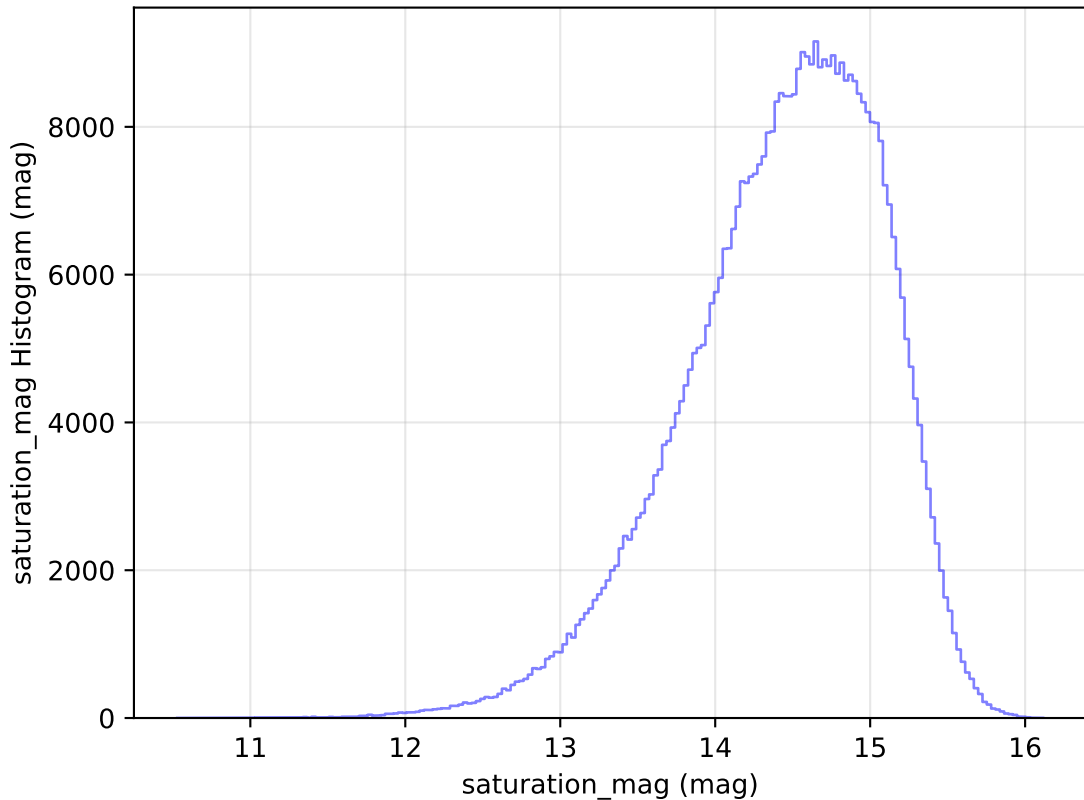
ddf_loaded_fl15_v3.4_10yrs All sky i band: saturation_mag Histogram
