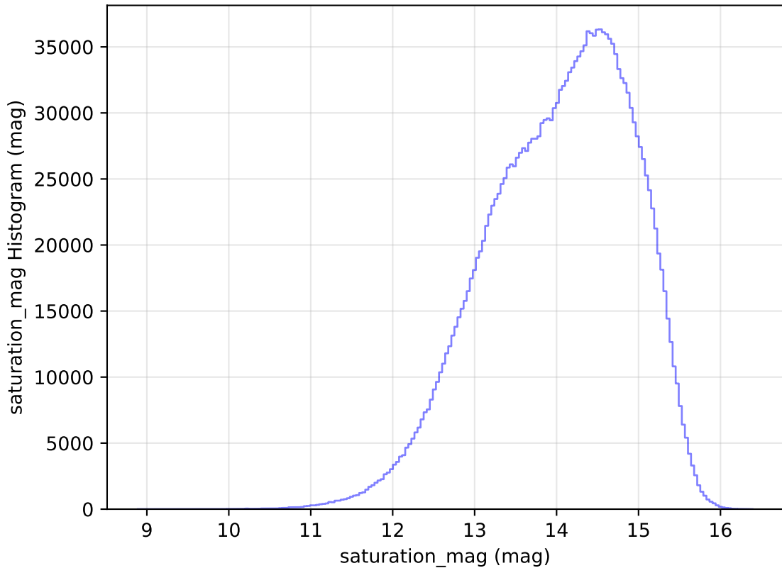
ddf_loaded_fl15_v3.4_10yrs All sky all bands: saturation_mag Histogram
