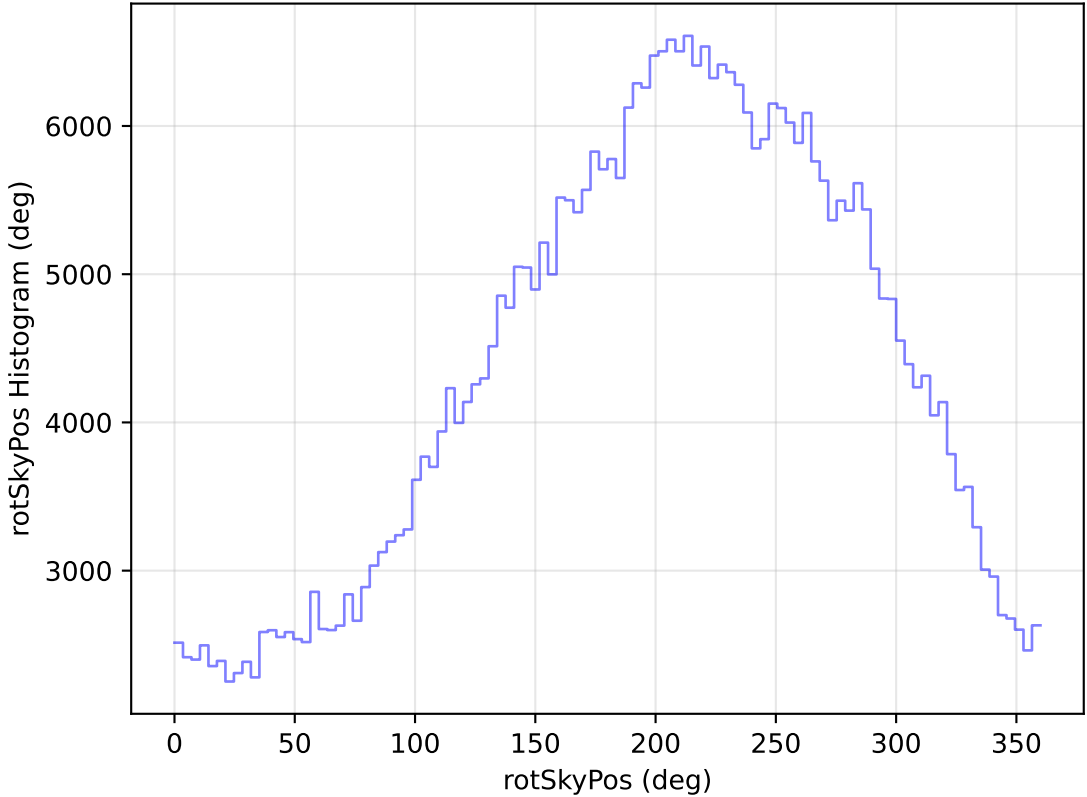
ddf_loaded_fl15_v3.4_10yrs WFD z band: rotSkyPos Histogram
