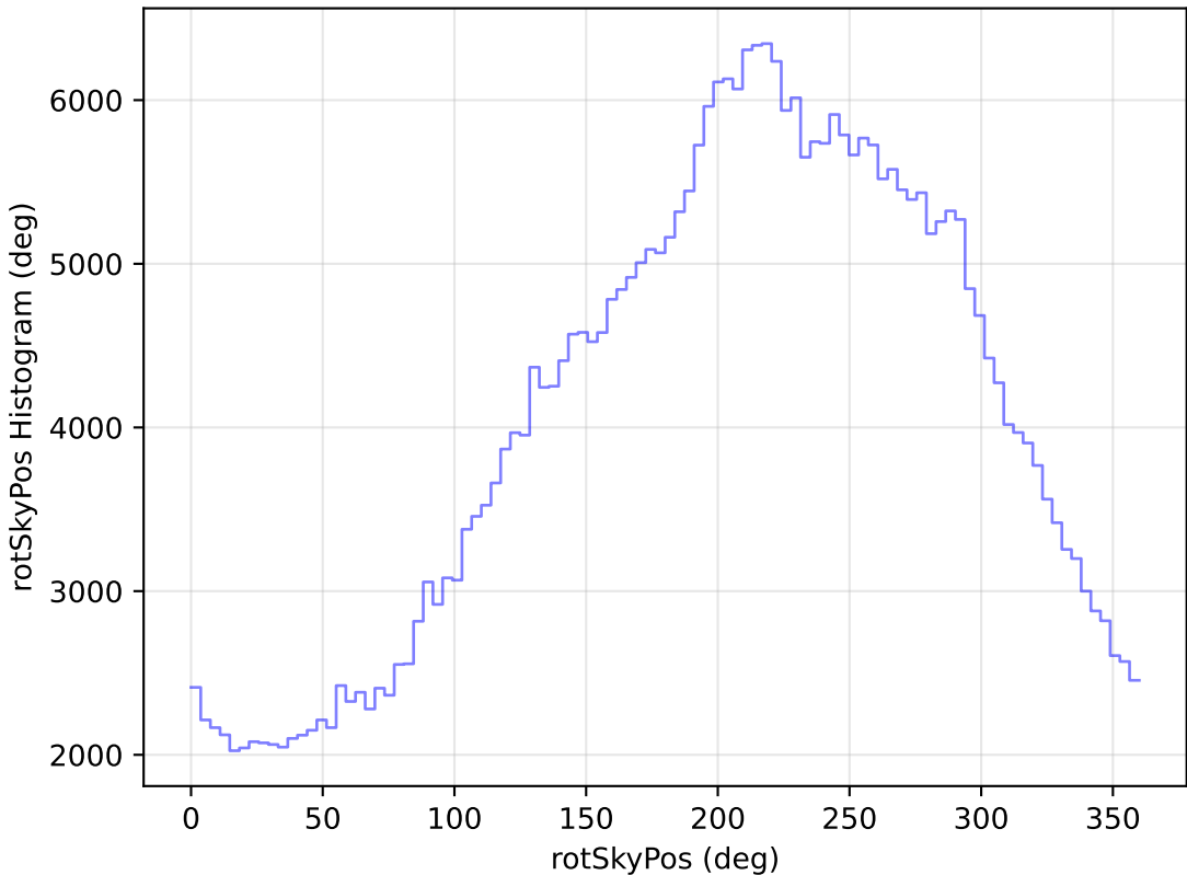
ddf_loaded_fl15_v3.4_10yrs WFD y band: rotSkyPos Histogram
