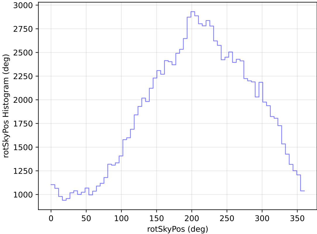
ddf_loaded_fl15_v3.4_10yrs WFD u band: rotSkyPos Histogram
