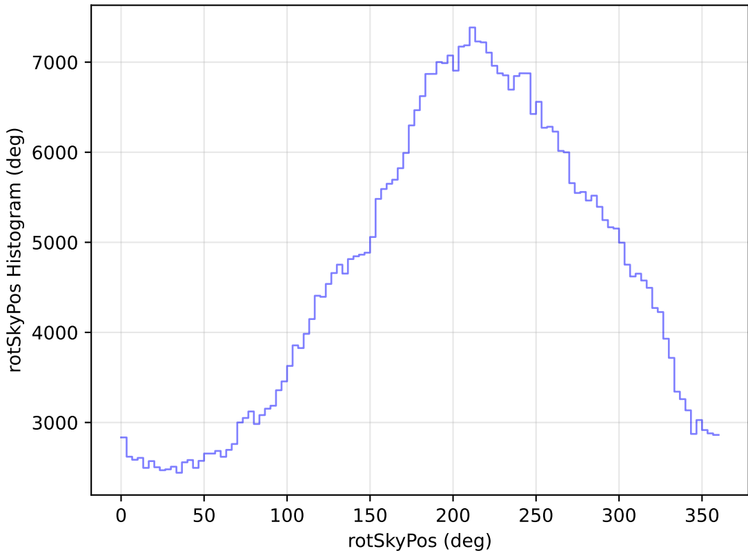
ddf_loaded_fl15_v3.4_10yrs WFD i band: rotSkyPos Histogram
