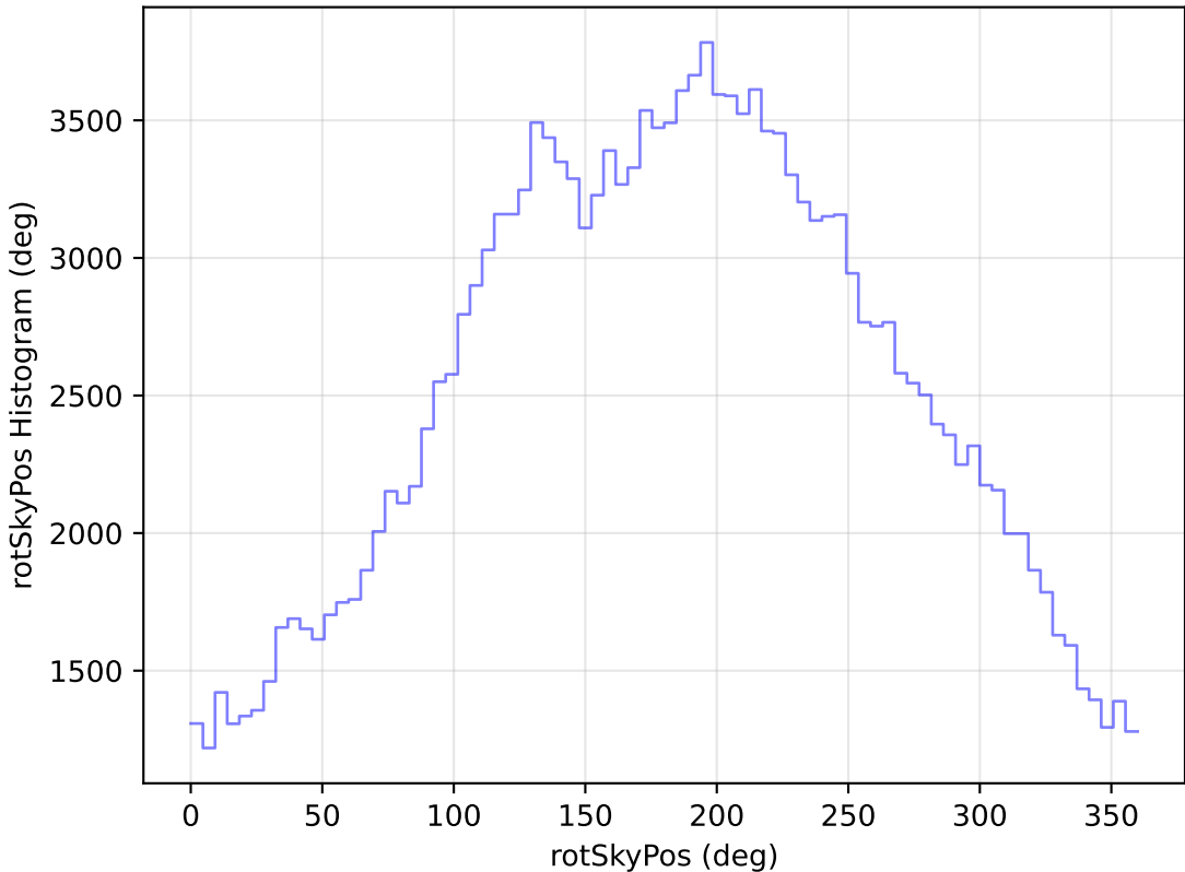
ddf_loaded_fl15_v3.4_10yrs WFD g band: rotSkyPos Histogram
