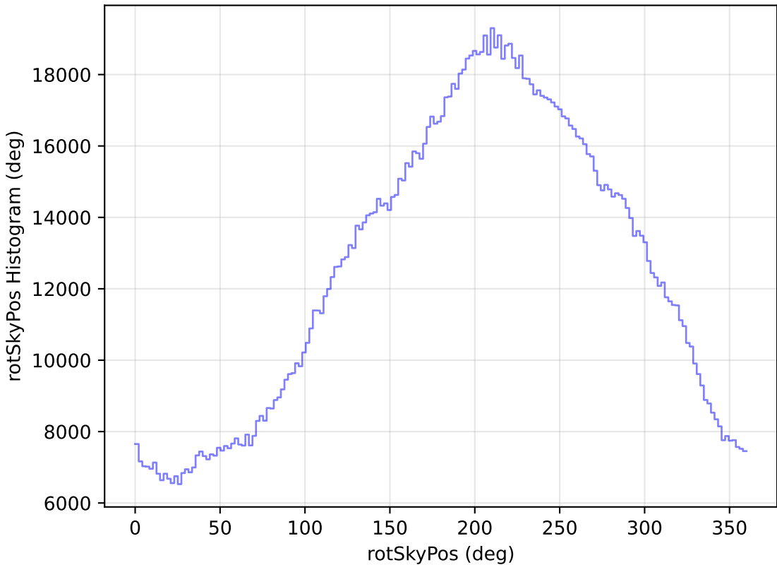
ddf_loaded_fl15_v3.4_10yrs WFD all bands: rotSkyPos Histogram
