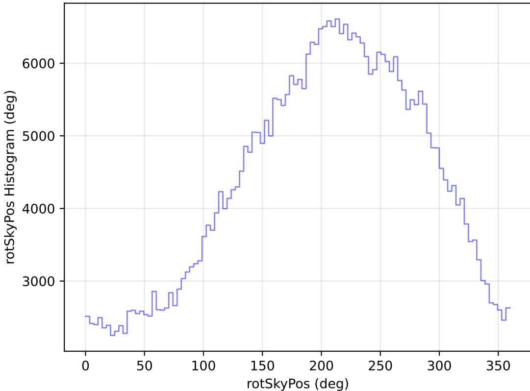
ddf_loaded_fl15_v3.4_10yrs All sky z band: rotSkyPos Histogram
