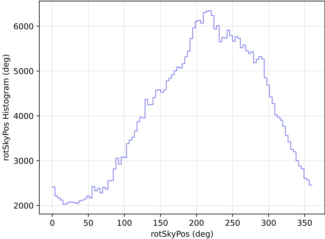
ddf_loaded_fl15_v3.4_10yrs All sky y band: rotSkyPos Histogram
