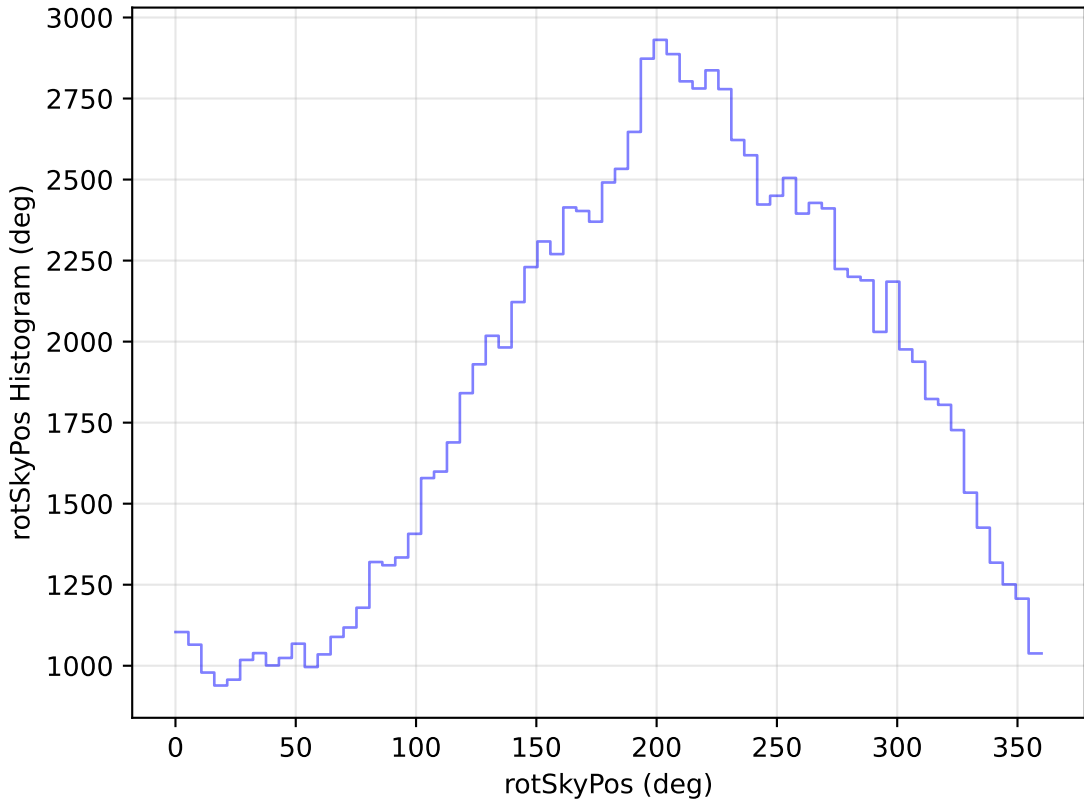
ddf_loaded_fl15_v3.4_10yrs All sky u band: rotSkyPos Histogram
