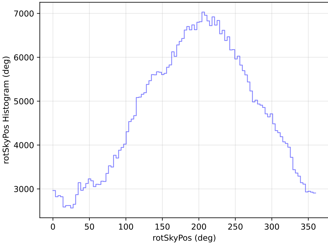
ddf_loaded_fl15_v3.4_10yrs All sky r band: rotSkyPos Histogram
