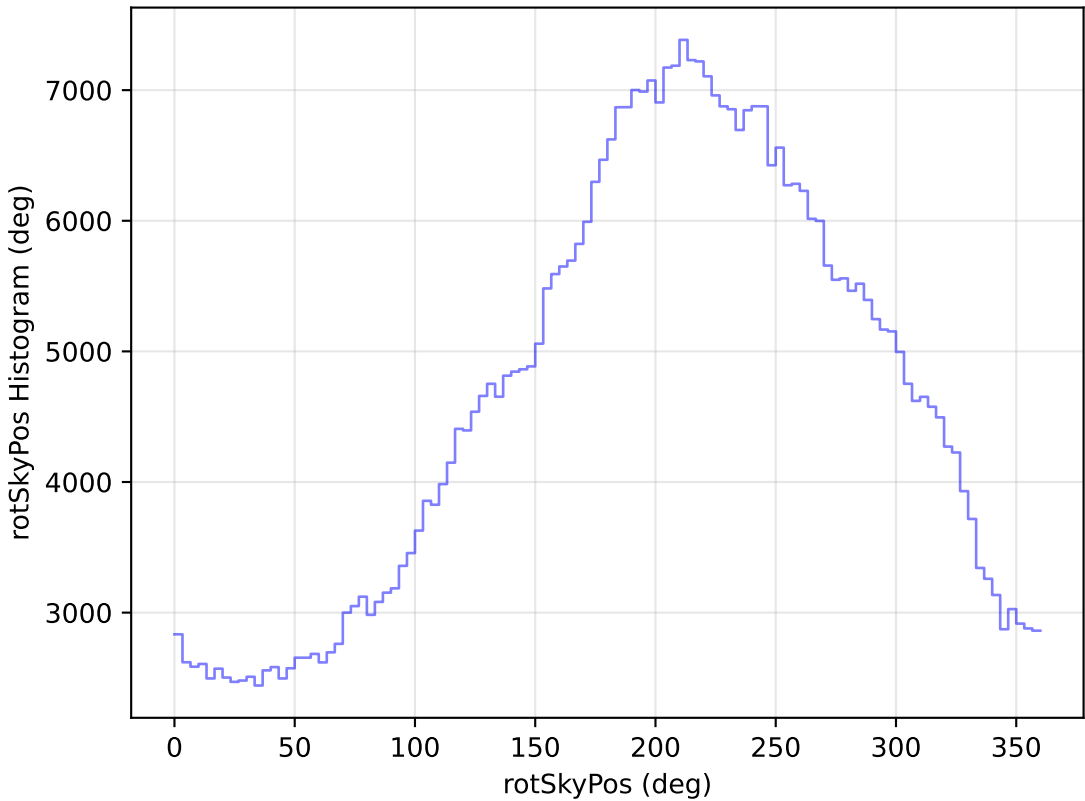
ddf_loaded_fl15_v3.4_10yrs All sky i band: rotSkyPos Histogram
