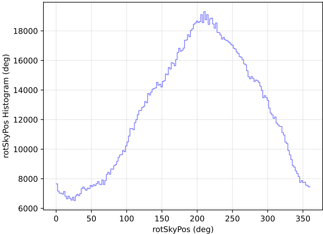
ddf_loaded_fl15_v3.4_10yrs All sky all bands: rotSkyPos Histogram
