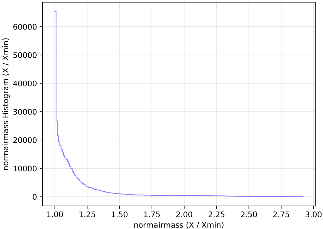
ddf_loaded_fl15_v3.4_10yrs WFD z band: normairmass Histogram
