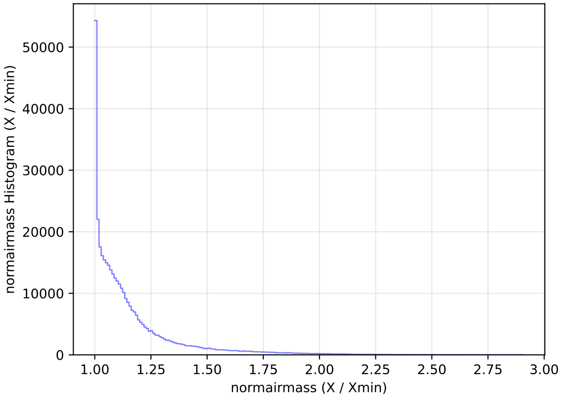
ddf_loaded_fl15_v3.4_10yrs WFD y band: normairmass Histogram
