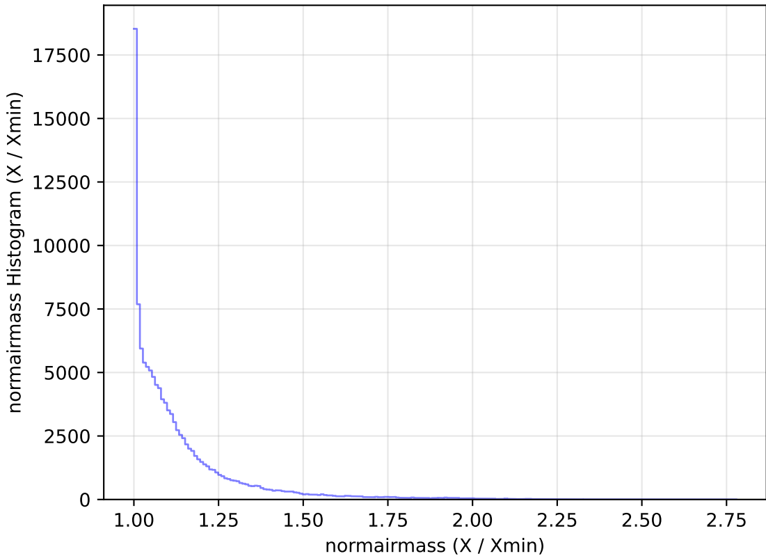
ddf_loaded_fl15_v3.4_10yrs WFD u band: normairmass Histogram
