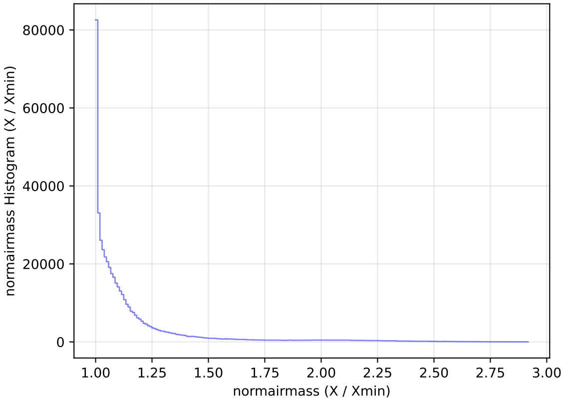
ddf_loaded_fl15_v3.4_10yrs WFD i band: normairmass Histogram
