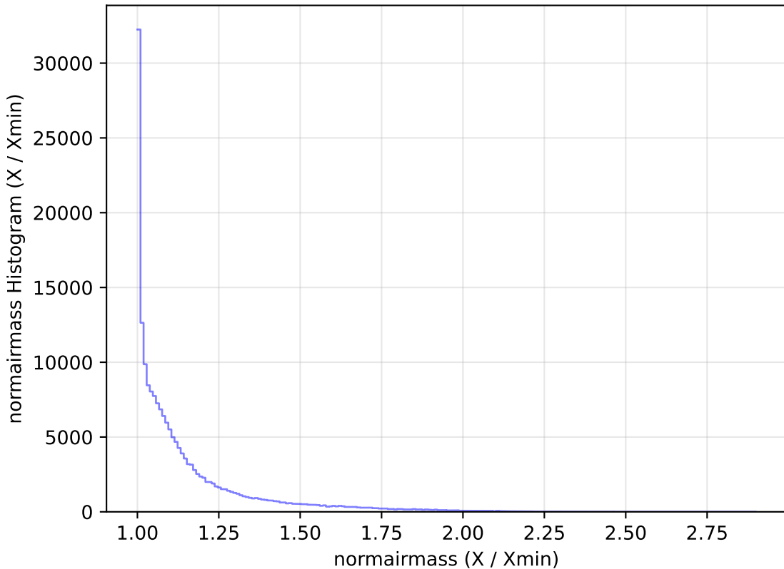
ddf_loaded_fl15_v3.4_10yrs WFD g band: normairmass Histogram
