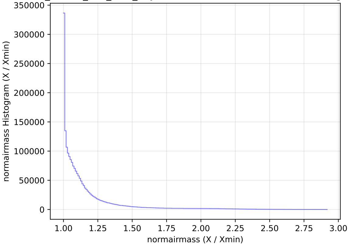
ddf_loaded_fl15_v3.4_10yrs WFD all bands: normairmass Histogram
