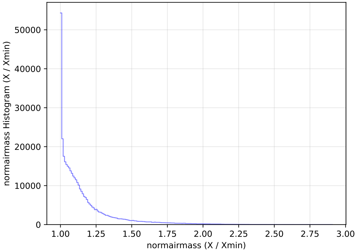
ddf_loaded_fl15_v3.4_10yrs All sky y band: normairmass Histogram
