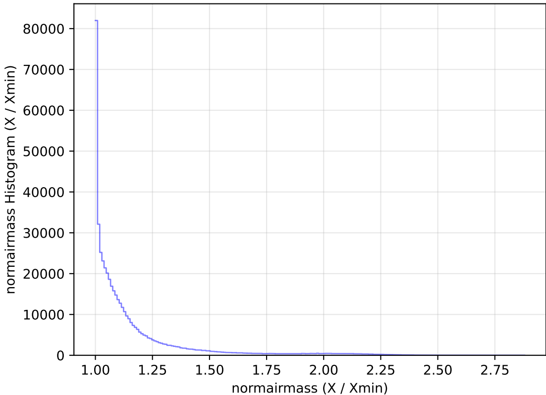
ddf_loaded_fl15_v3.4_10yrs All sky r band: normairmass Histogram
