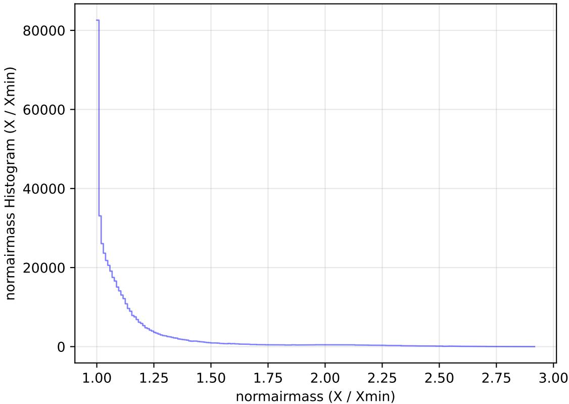
ddf_loaded_fl15_v3.4_10yrs All sky i band: normairmass Histogram
