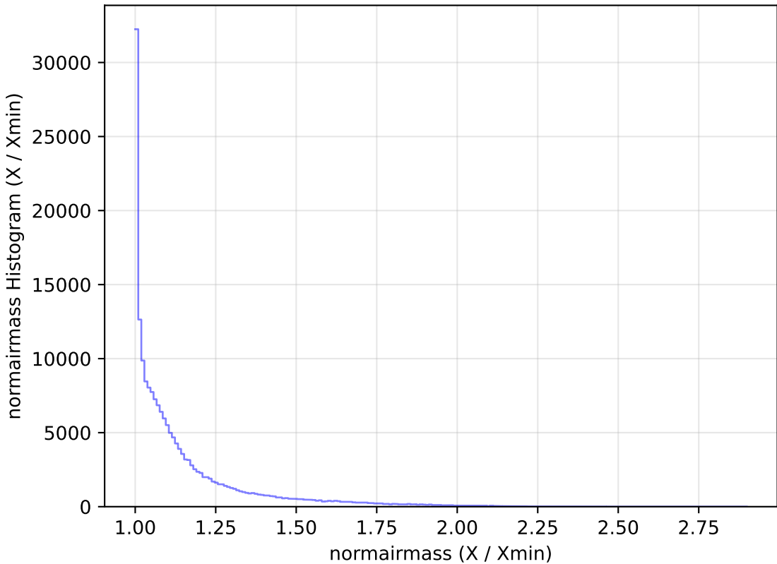
ddf_loaded_fl15_v3.4_10yrs All sky g band: normairmass Histogram
