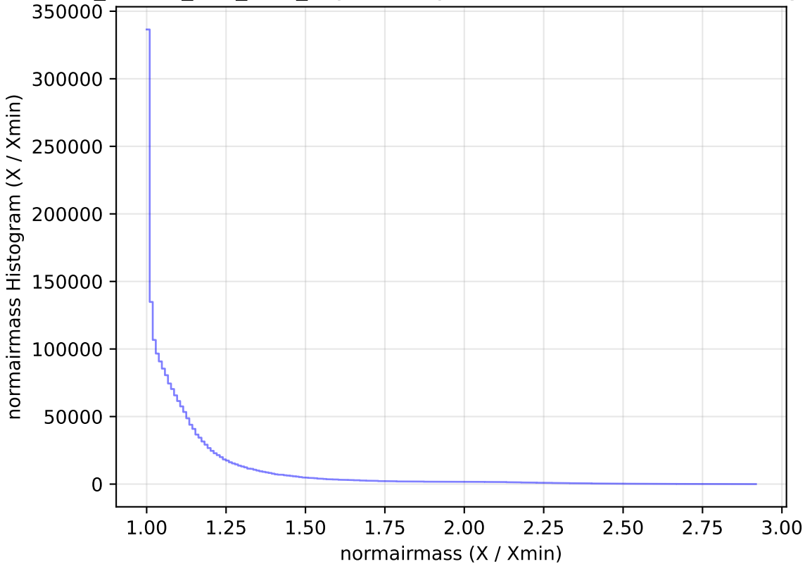
ddf_loaded_fl15_v3.4_10yrs All sky all bands: normairmass Histogram
