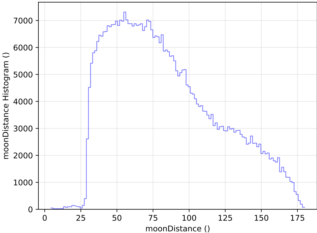
ddf_loaded_fl15_v3.4_10yrs WFD z band: moonDistance Histogram
