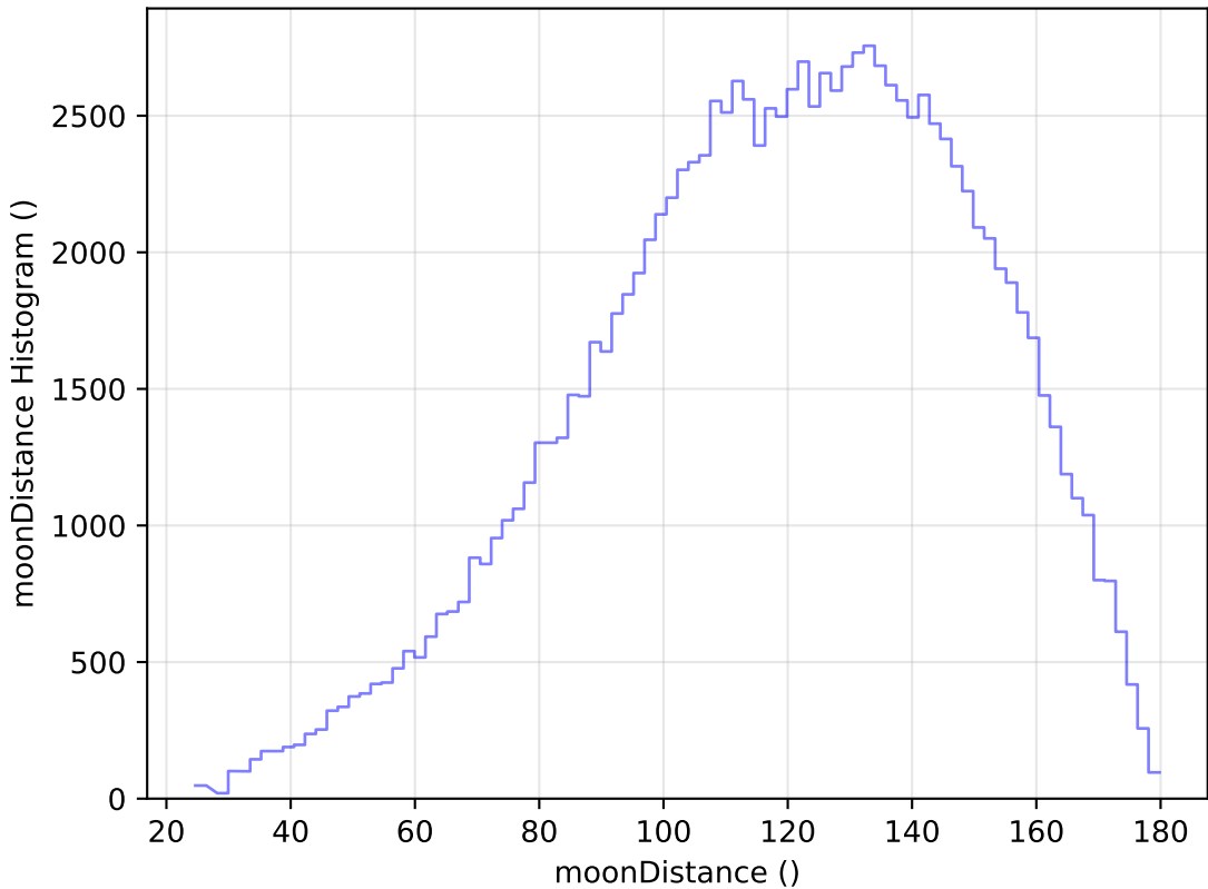
ddf_loaded_fl15_v3.4_10yrs WFD u band: moonDistance Histogram
