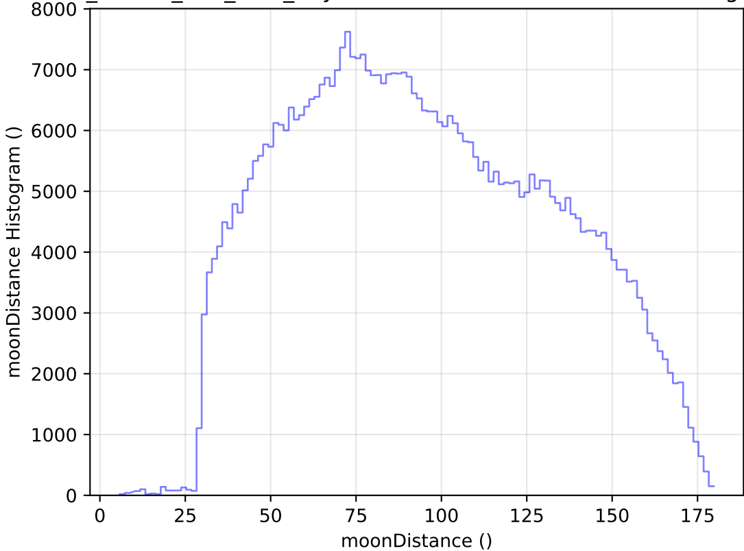
ddf_loaded_fl15_v3.4_10yrs WFD i band: moonDistance Histogram
