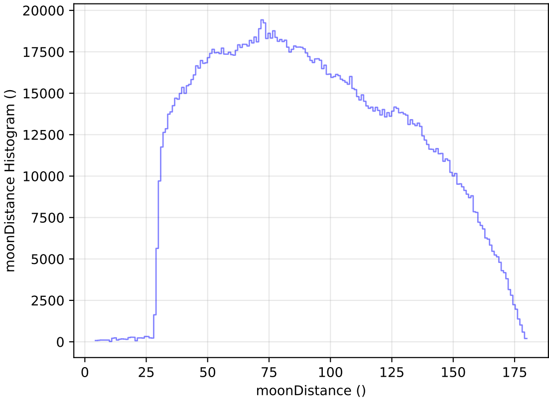
ddf_loaded_fl15_v3.4_10yrs WFD all bands: moonDistance Histogram
