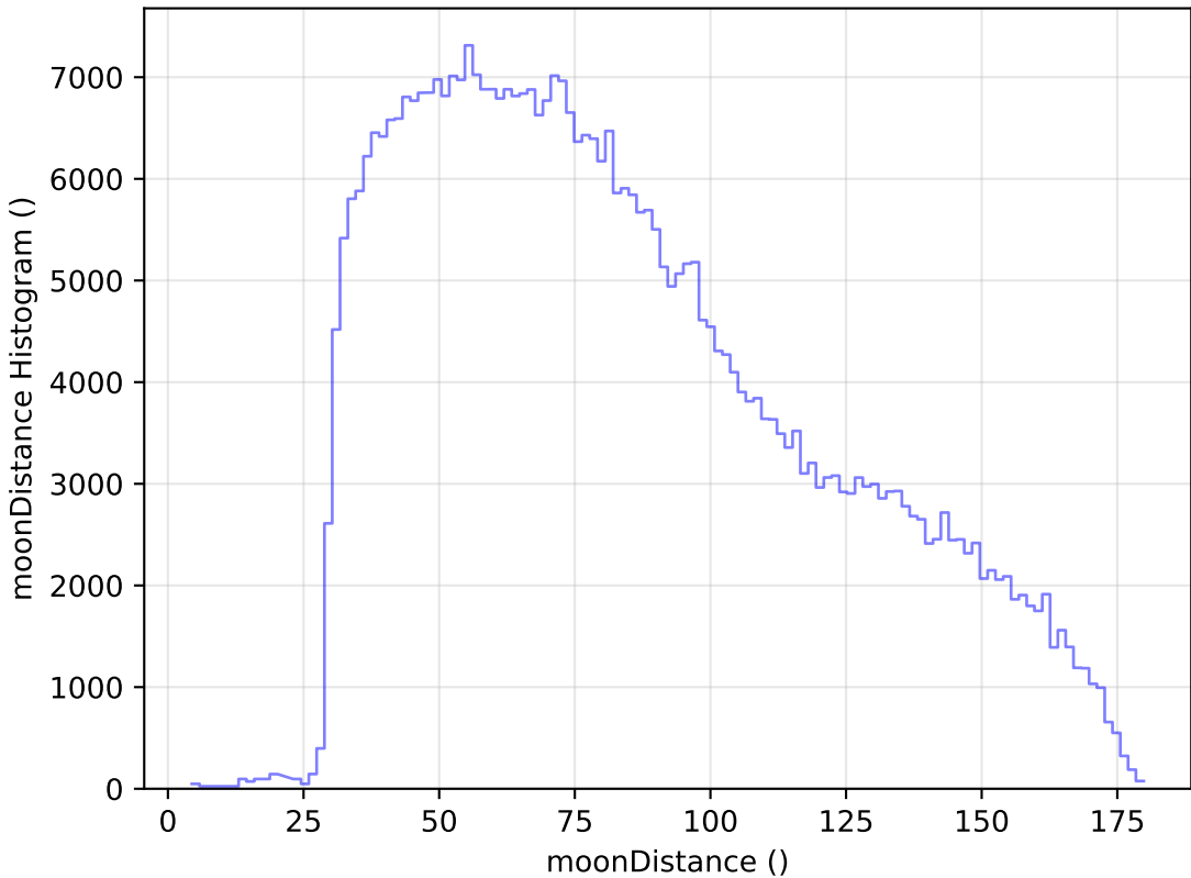
ddf_loaded_fl15_v3.4_10yrs All sky z band: moonDistance Histogram
