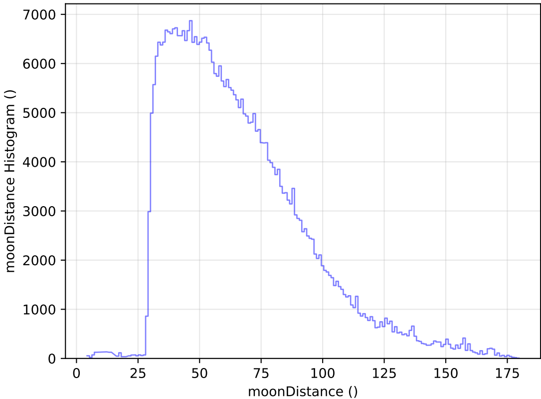
ddf_loaded_fl15_v3.4_10yrs All sky y band: moonDistance Histogram
