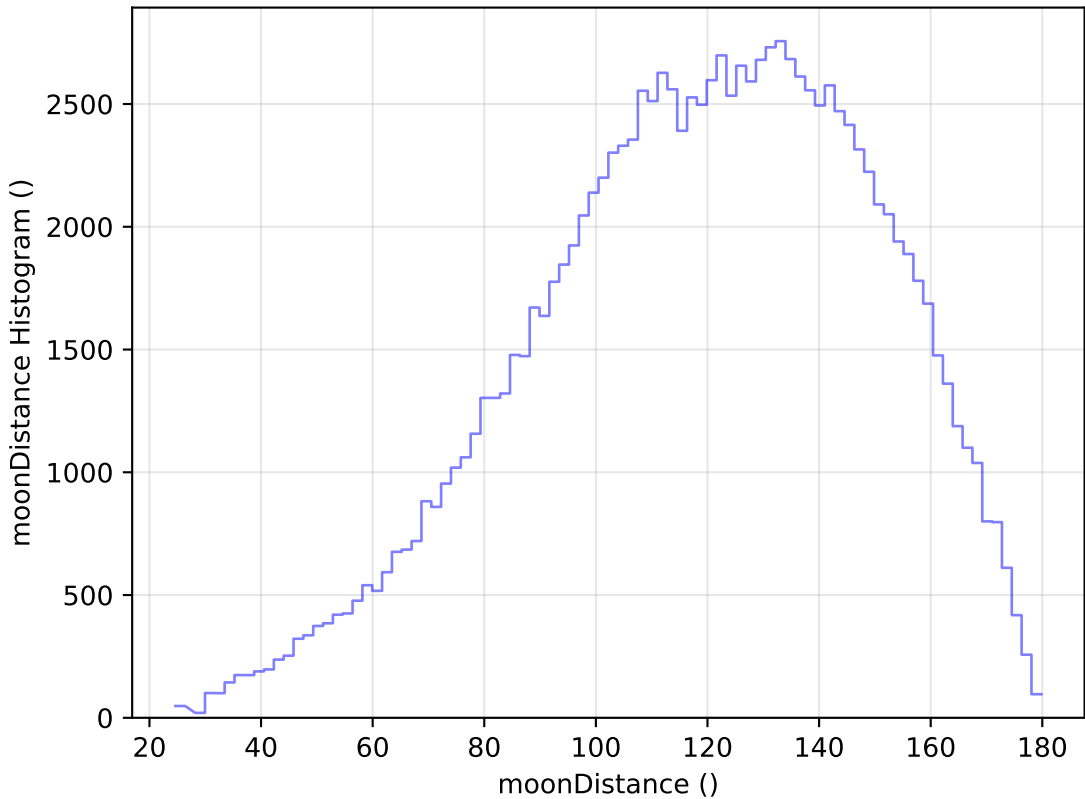
ddf_loaded_fl15_v3.4_10yrs All sky u band: moonDistance Histogram
