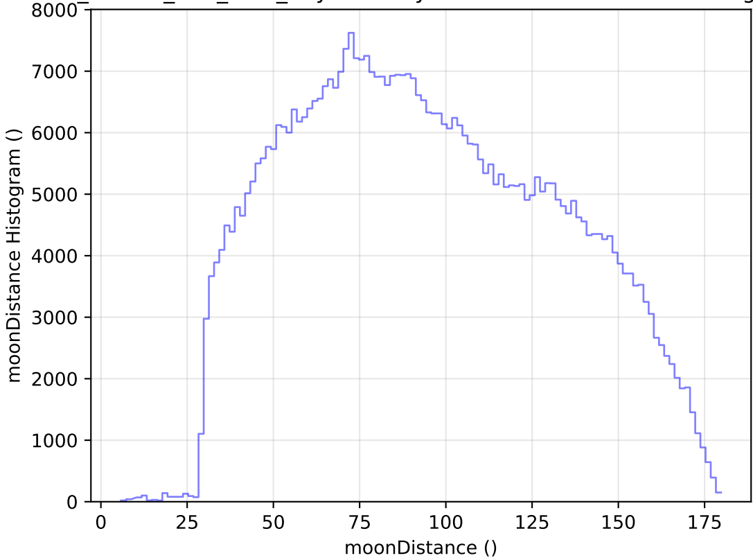
ddf_loaded_fl15_v3.4_10yrs All sky i band: moonDistance Histogram
