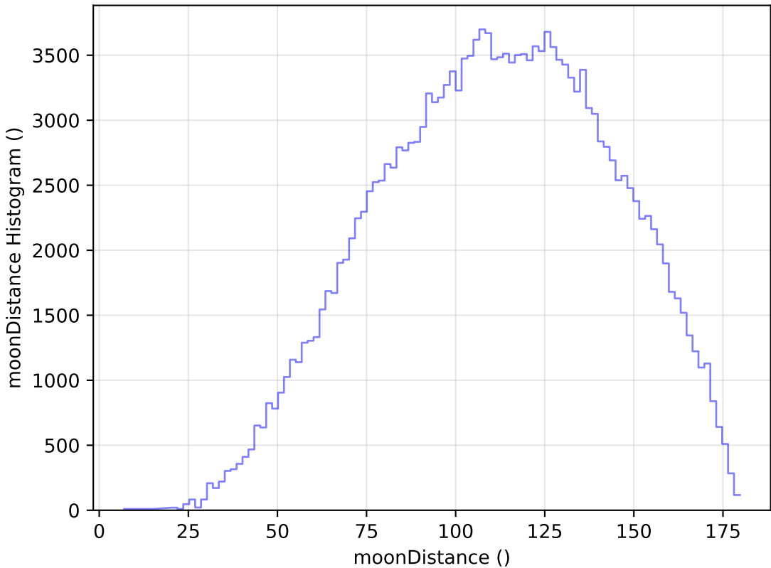
ddf_loaded_fl15_v3.4_10yrs All sky g band: moonDistance Histogram
