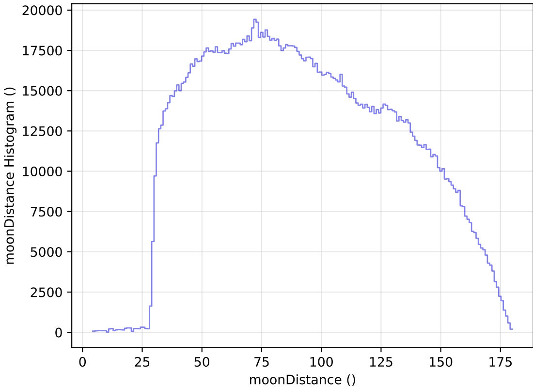
ddf_loaded_fl15_v3.4_10yrs All sky all bands: moonDistance Histogram
