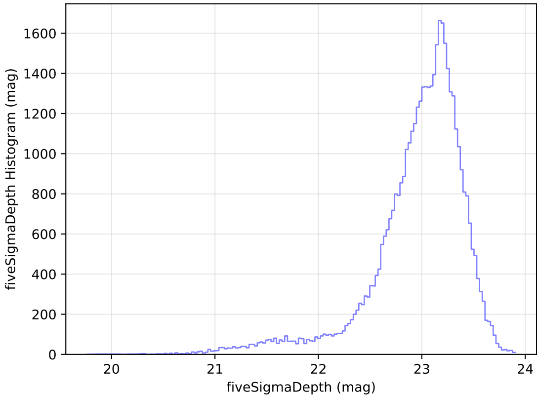
ddf_loaded_fl15_v3.4_10yrs Yr 1 z band: fiveSigmaDepth Histogram
